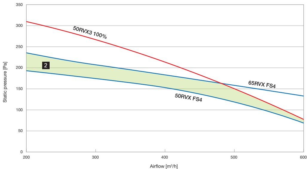
2 Where 65RVX was previously chosen, 50RVX3 (one size down) may now be chosen, owing to its increased external static pressure.
